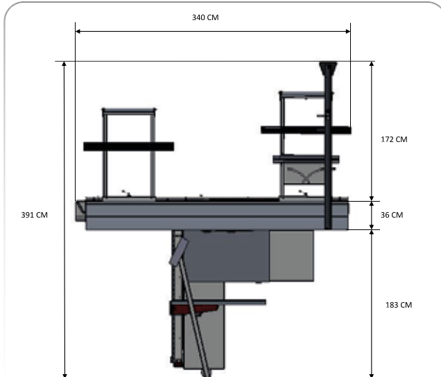
FUL OTOMATİK ÇİZİCİLİ YATAR DAİRE MAKİNASI 3800 YERLEŞİM PLANI FULL AUTOMATIC CIRCULAR SAW 3800 LAYOUT PLAN
